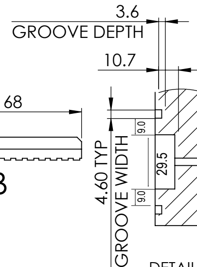
DETAIL C SCALE 1 : 2
